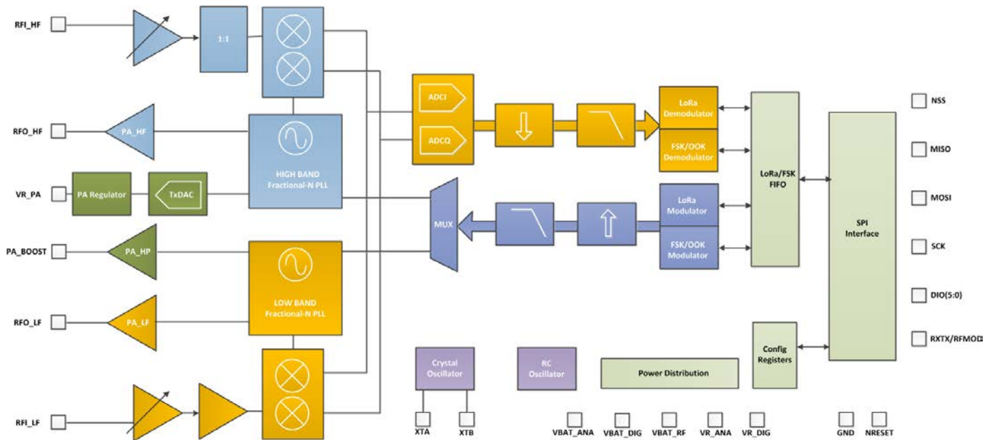
Figure 1. Block Diagram
